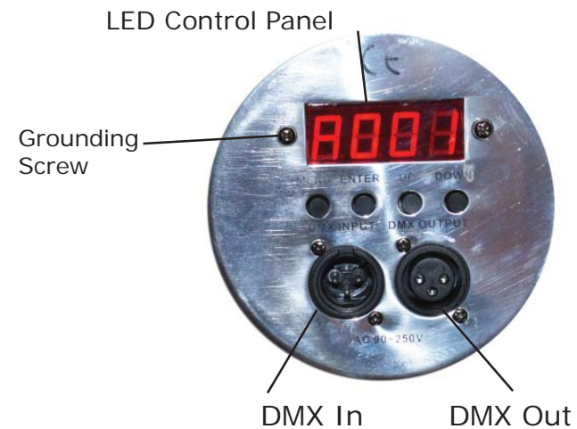
Figure 2: The Rear Connections
