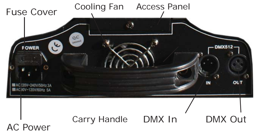
Figure 2: The Rear Connections
